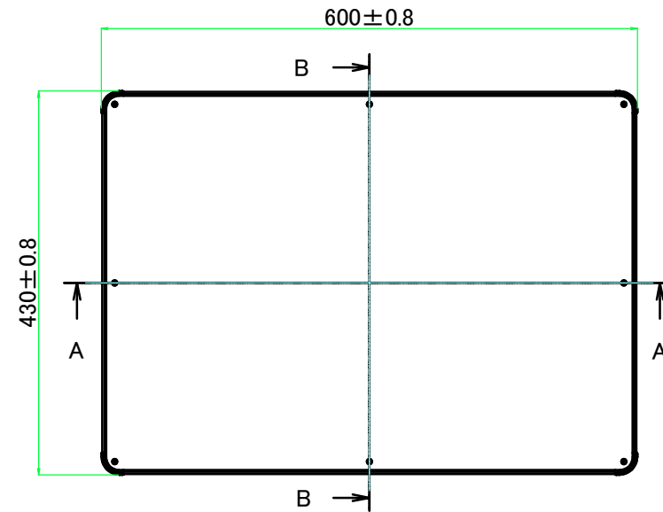
E view
